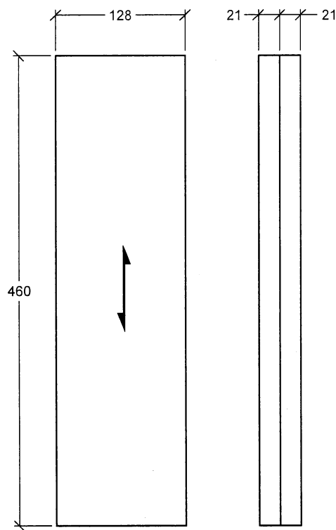
SEAT PANEL SOLID BEECH 2 PC/SET
