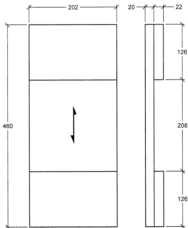
SEAT PANEL SOLID BEECH 1 PC/SET
