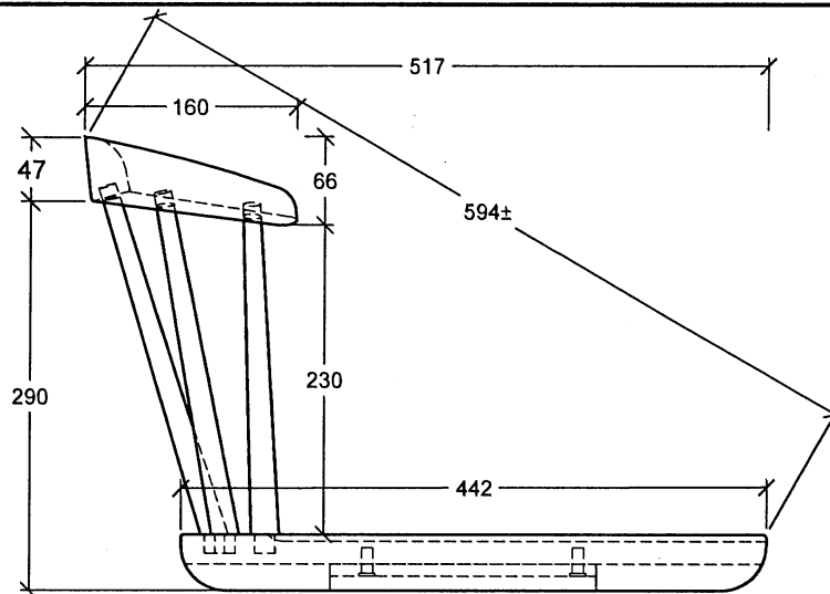
SEAT FRAME SOLID BEECH + PLYWOOD 1 Pc/set
